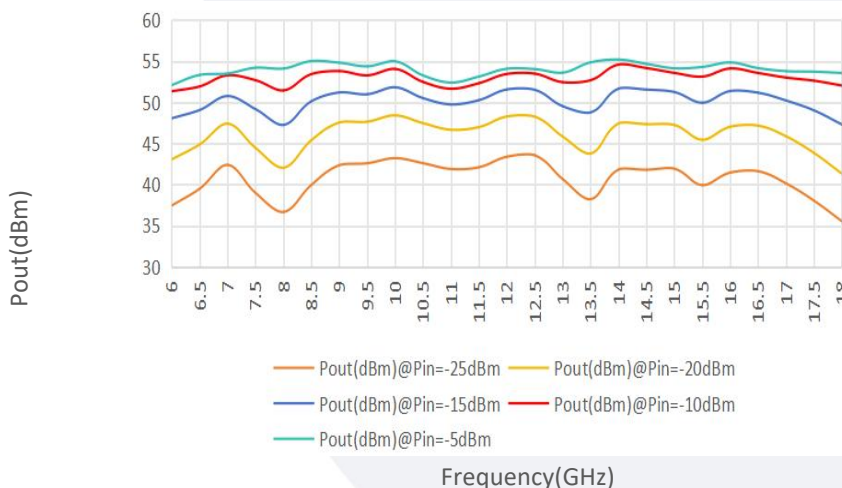
Pout@Equal_Pin
