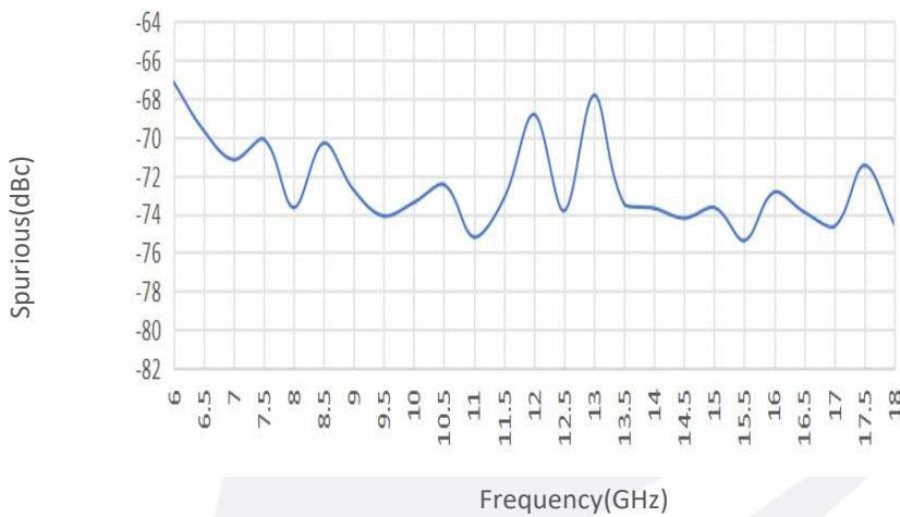
Harmonic@Pout=50dBm
