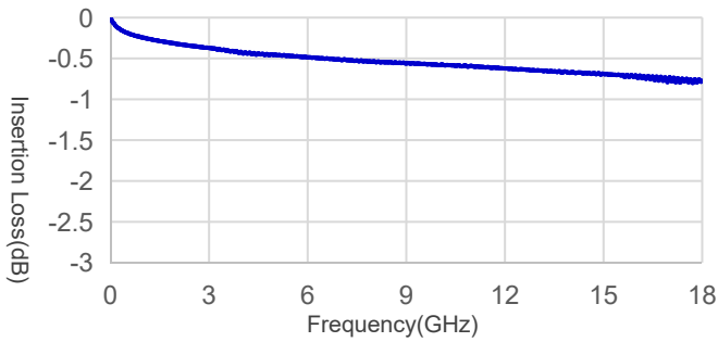
A81-NMNWM-1m Insertion Loss
