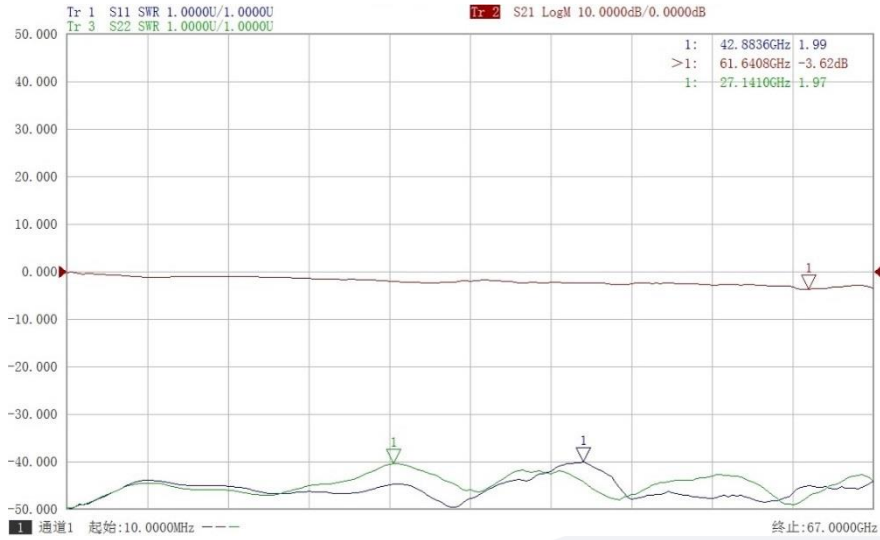
Insertion Loss&VSWR vs Frequency
