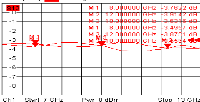
Trc3 S12 dB Mag 1 dB / Ref -3 dB Cal 3 Mem5[Trc3] S12 dB Mag 1 dB / Ref -3 dB
