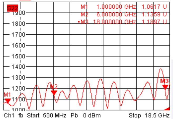
Trc4 S22 SWR 100 mU/ Ref1 U Cal 4
