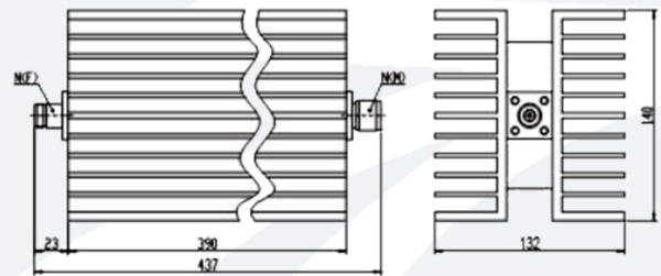
Connector: N and DIN 7/16 are optional. Unit:mm
