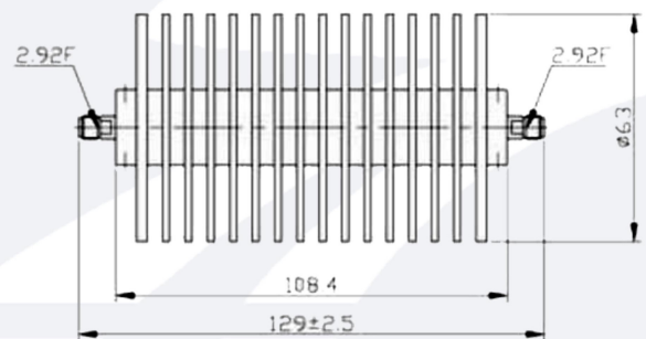
Connector: SMA , 3.5mm and K are optional. Unit:mm
