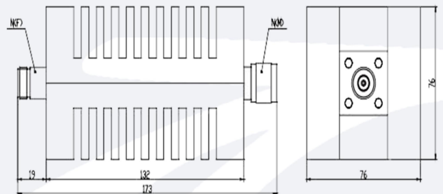
Connector: SMA and N are optional. Unit:mm
