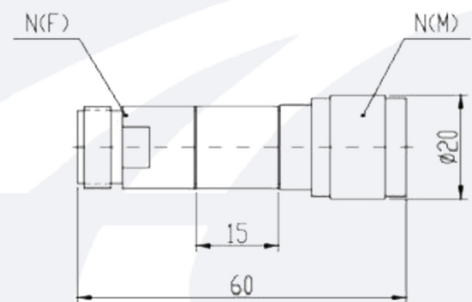
Connector: N and TNC are optional. Unit : mm
